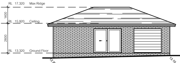
EAST ELEVATION
