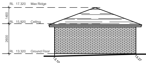
NORTH ELEVATION
