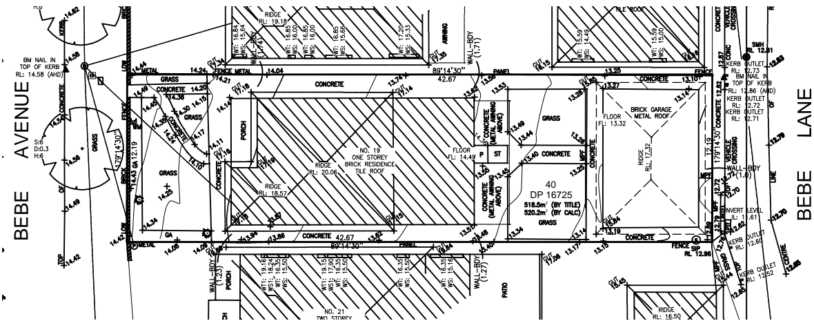
SITE PLAN
