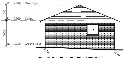
SOUTH ELEVATION
